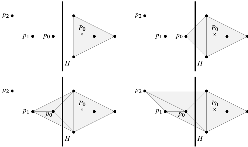
Figure 1. Regular subdivisions of a polytope in the proof of Lemma 2.16.
