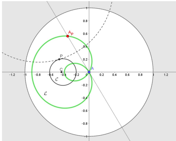
Figure 1. Hyperbolic limaçon for n = 2 , a > c .
