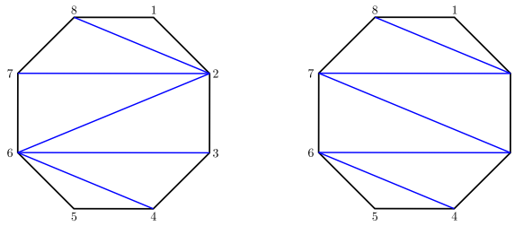
Figure 18. An edge flip at the diagonal D_{2,6} in the triangulation \mathcal{T}_{154362} yields the permutation 154632.
