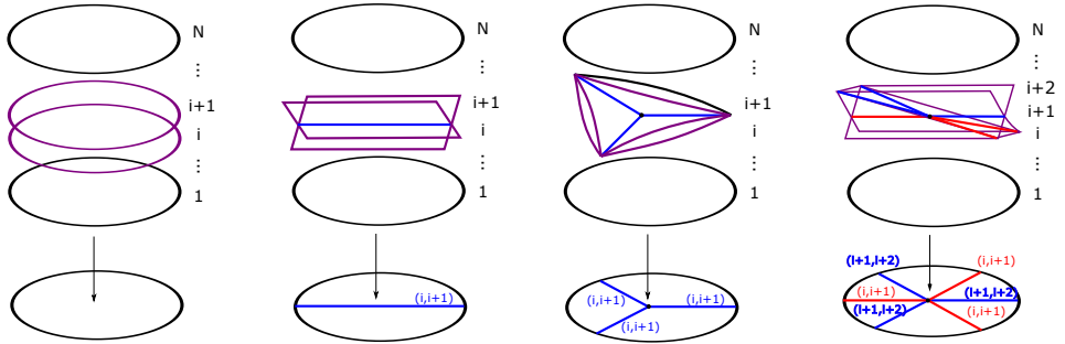
Figure 3. The weaving of singularities of fronts along the edges of the N -graph (courtesy of Roger Casals and Eric Zaslow, used with permission). Gluing these local models according to the N -graph \Gamma yields the weave \Lambda(\Gamma) .
