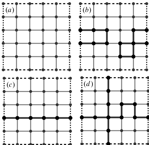
Figure 2. (a) A square tiling of the torus. The opposite boundaries are identified. (b) A cycle which is a boundary. (c) A cycle which is not a boundary. (d) A cycle which is not a boundary.
