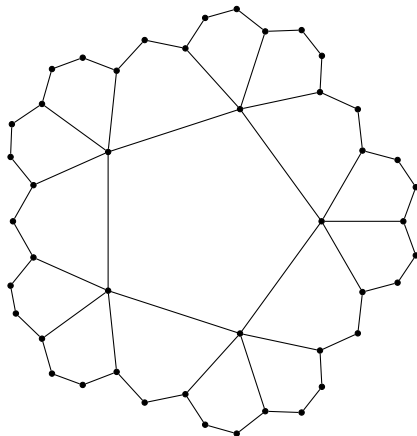
Figure 1. The local structure of the graph G(5)
