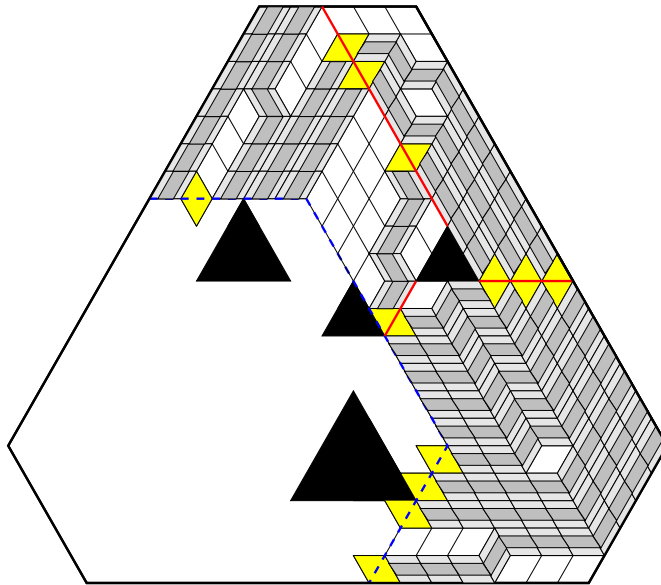
Figure 8. Proving polynomiality in b_2 . The region R on the lower left delimited by the dashed line does not change as b_2 varies; the lozenges that straddle the dashed line in one of its fixed number (independent of b_2 ) of tilings are indicated. The number of ways each such tiling of R can be extended to a tiling of S_{n_1, n_2, n_3, a, b_1, b_2, b_3, k_1, k_2, k_3} is polynomial in b_2 for fixed n_1, n_2, n_3, a, b_1, b_3, k_1, k_2, k_3 , by the argument in [18].
