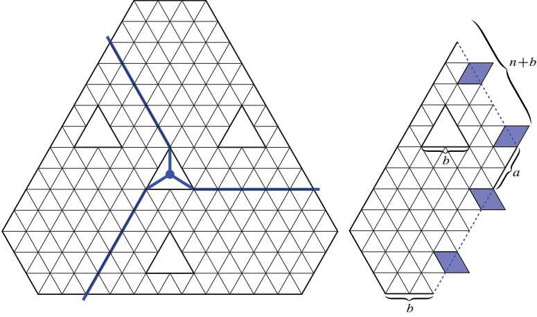
Figure 10. Applying equation (7.4) to the region S_{n,a,b,k} (left; here n = 3, a = 2, b = 2 and k = 1 ). The region whose planar dual is G_1 (right; the dotted portions of the boundary are glued together).
