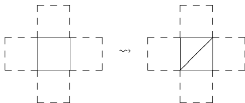
FIG. 3. A quadric degenerating to the union of two planes.
