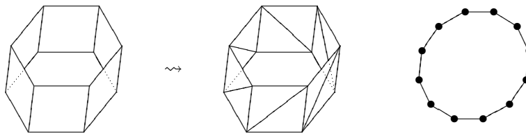
FIG. 6. Cycle of n quadrics and of 2n planes as in Example 3.3.
