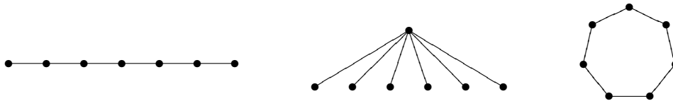
FIG. 1. A chain R_n , a fork S_n with n - 1 teeth, a cycle E_n .
