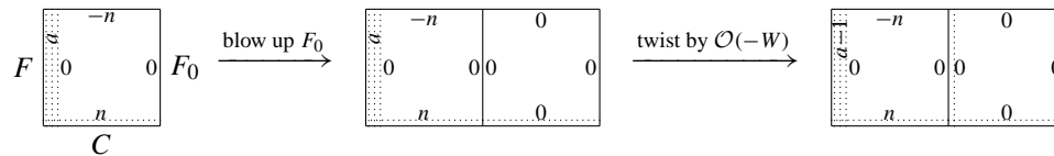
FIG. 9. Degeneration of a scroll S_{a,b} to the union of a quadric and a scroll S_{a-1,b-1} .
