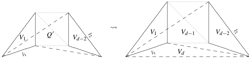
FIG. 13. Construction of X_{d,1} from X_{d-2,0} .
