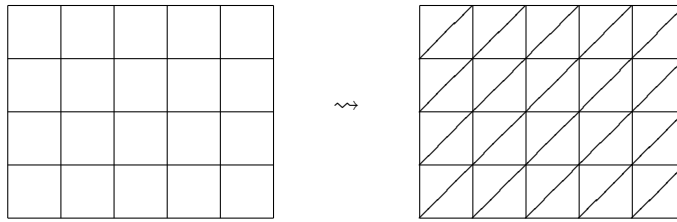
FIG. 7. nm quadrics with E_4 -points and 2nm planes with E_6 -points.
