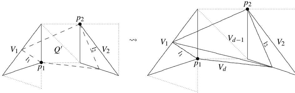
FIG. 14. Construction of X_{d,g} from X_{d-2,g-1} .
