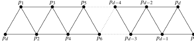
FIG. 12. Planar Zappatic surface X_{d,1} with dual graph a cycle.
