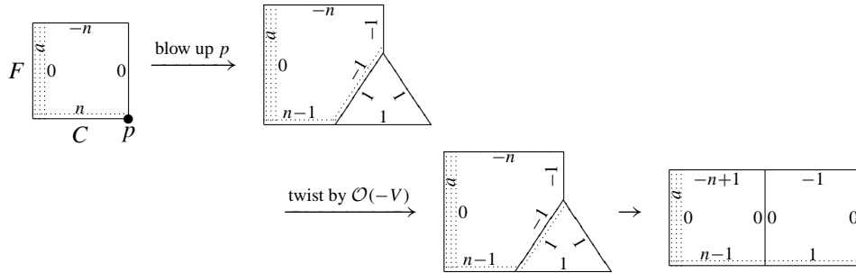
FIG. 8. Degeneration of a scroll S_{a,b} to the union of a plane and a scroll S_{a,b-1} .
