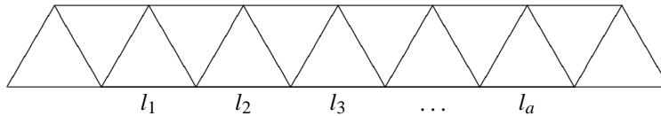
FIG. 11. Degeneration of S_{a,b} , b = a + 3 , to X with only R_3 -points.
