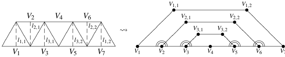
FIG. 15. Construction of Y_{d,g} from X_{d-2g,0} for g = 3 and d = 4g + 1 = 13 .
