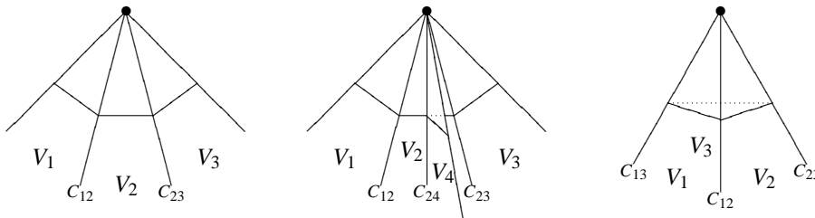
FIG. 2. Examples: an R_3 -point, an S_4 -point and an E_3 -point.
