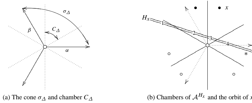
FIG. 1. The A_2 root system
