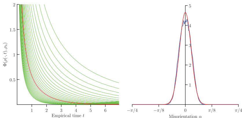
Figure 6. Average over 10 1D trials with 2^{15} initial grain boundaries: (a) Relative entropy curves \Phi_\lambda(\rho(\cdot, t), \rho_\sigma) for 30 uniformly spaced trial values \lambda \in [0.01, 0.05] . The red curve depicts the optimal curve for \sigma \approx 0.02931 . (b) Comparison of the steady-state GBCD (80% removal) and the exact Boltzmann distribution \rho_\sigma for the obtained \sigma \approx 0.02931 .
