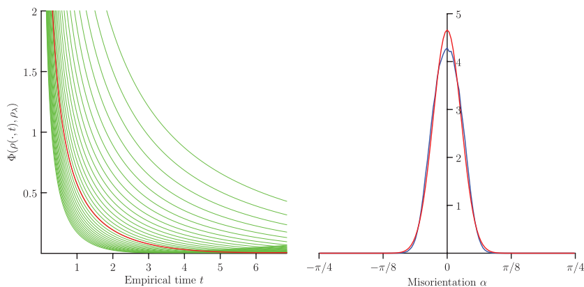
Figure 11. Average over 10 1D trials with 2^{18} initial grain boundaries: (a) Relative entropy curves \Phi_\lambda(\rho(\cdot, t), \rho_\lambda) for 30 uniformly spaced trial values \lambda \in [0.01, 0.05] . The red curve depicts the optimal curve for \sigma \approx 0.02931 . (b) Comparison of the steady-state GBCD (80% removal) and the optimal Boltzmann distribution \rho_\sigma .
