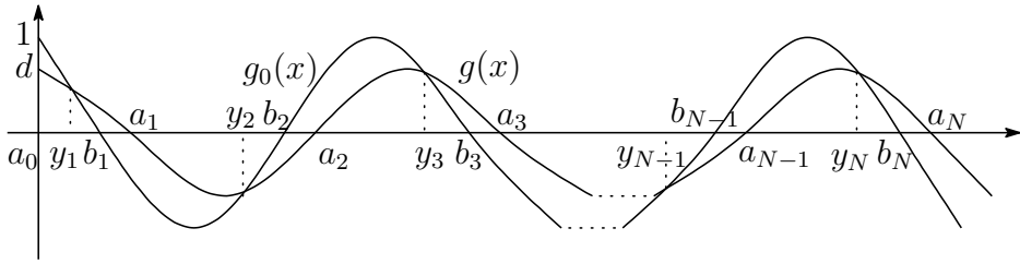
FIGURE 3. Two functions g(x) and g_0(x) .
