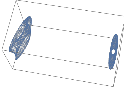
FIGURE 1. Two Siegel disks for automorphism F .
