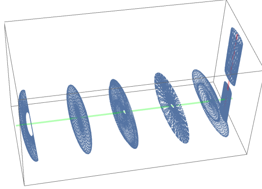
FIGURE 2. Siegel disks for an automorphism ( N = 5 ).
