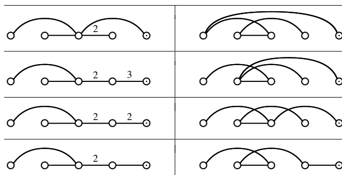
Fig. 11. Building a bijection between labeled floor diagrams and trees.
