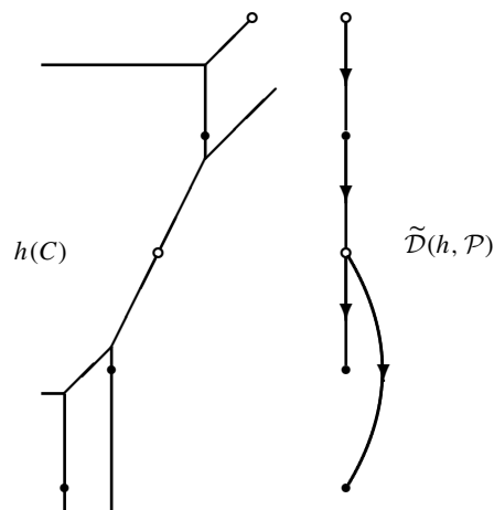
Fig. 5. Marked floor diagram of a tropical curve.
