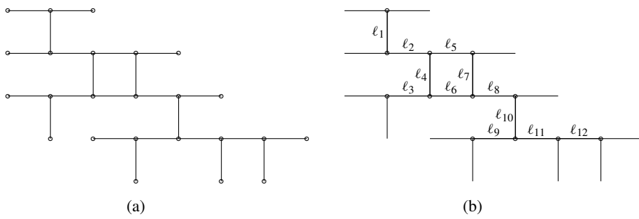
Fig. 3. A graph and a related tropical curve.
