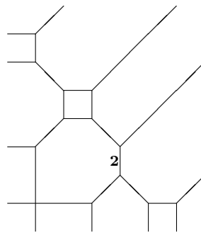
Fig. 4. The image of a plane tropical curve.
