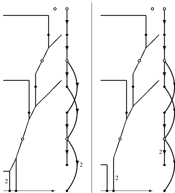
Fig. 6. Two tropical cubics passing through six vertically stretched points and (\lambda, \mathcal{P}_\lambda, \rho) -grounded with \lambda = \emptyset , \mathcal{P} = \emptyset , and \rho = (2, 1) . The multiplicity of each tropical cubic is 2; thus N_{3,1}(\emptyset, (2, 1)) = 4 .
