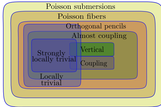
Figure 2. Hierarchy of Poisson submersions.
