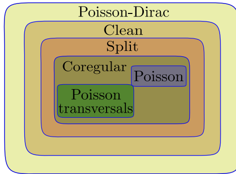
Figure 1. Hierarchy of induced Poisson structures.
