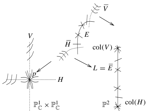
Figure 9. Passing from \mathbb{P}^1_{\mathbb{C}} \times \mathbb{P}^1_{\mathbb{C}} to \mathbb{P}^2 .
