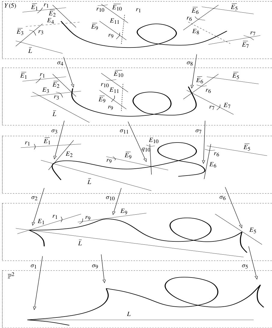
Figure 18. Resolution of \mathcal{H}_3 .
