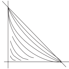
Figure 2. The qualitative behavior of \mathcal{H}_5 and \mathcal{H}_9 on each cell.
