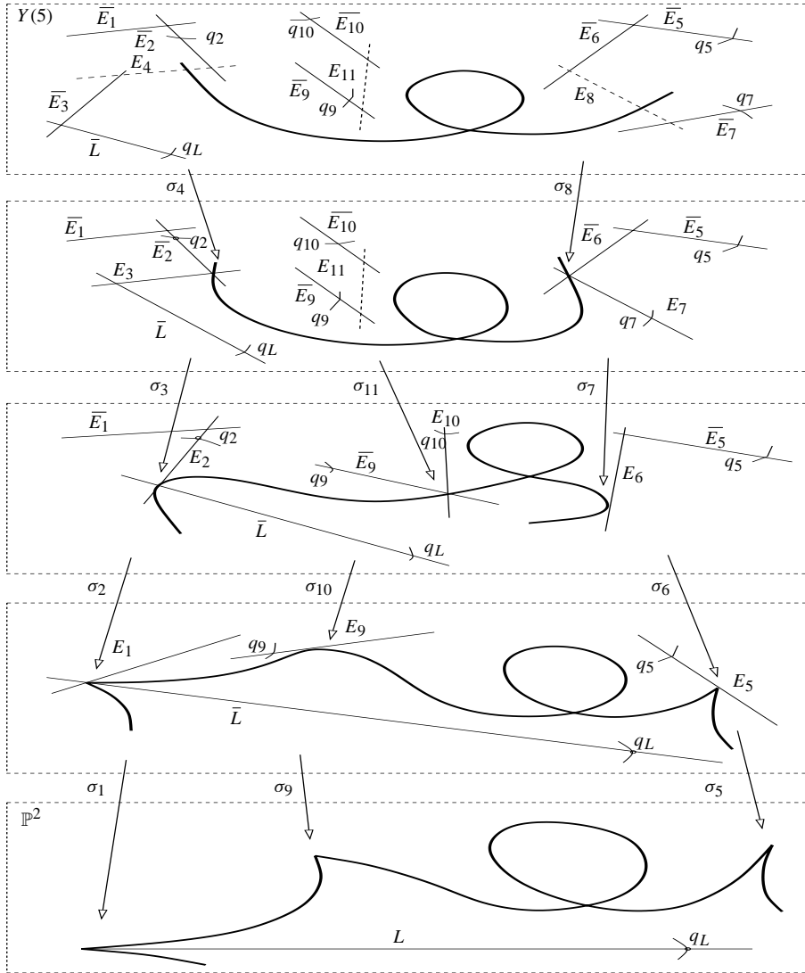
Figure 17. Resolution of \mathcal{H}_2 .
