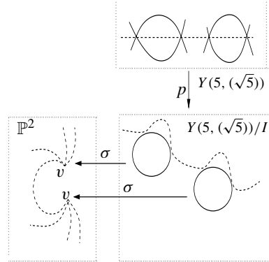
Figure 15. The 2-fold covering of Y(5, (\sqrt{5})) over the blown up plane.
