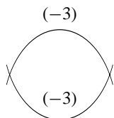
Figure 12. Cycles composed by two components on Y(5, (\sqrt{5})) .
