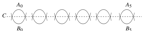
Figure 13. The resolution of cusps of Y(5, (\sqrt{5})) .
