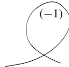
Figure 11. \bar{Q} \subset Y(5) is a cycle introduced in the resolution of the cusp.
