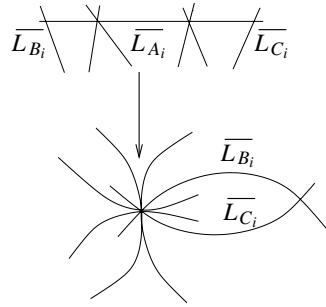
Figure 8. Contraction producing the point r_{A_i} of \mathbb{P}_{\mathbb{C}}^1 \times \mathbb{P}_{\mathbb{C}}^1 .
