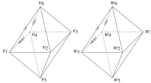
Figure 13. Configuration (A').
