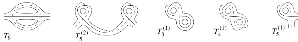
Figure 14. Particular triangulations or fragments of.
