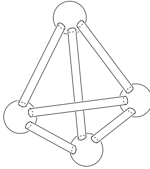
Figure 18. A handlebody.
