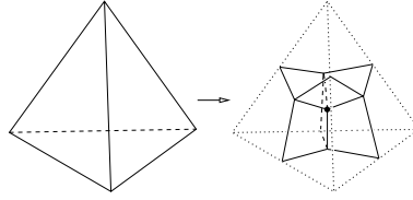
Figure 5. From a triangulation to the dual special polyhedron.
