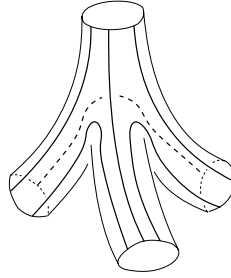
Figure 4. A tetrapod.
