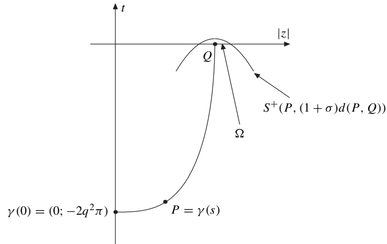
Figure 3. A bidimensional qualitative representation of inclusion (5.5).
