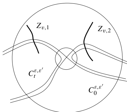
Figure 5. The sets Z_{v,i} .
