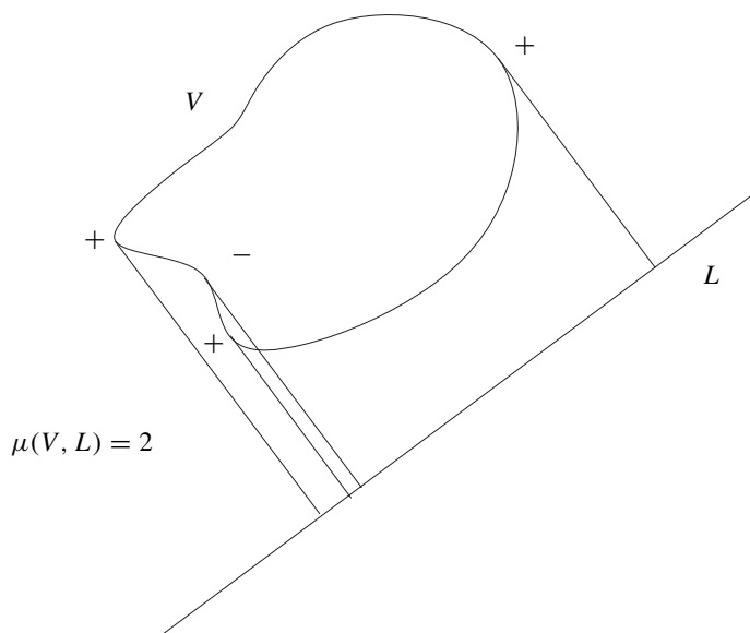
Figure 1. The exchange principle.
