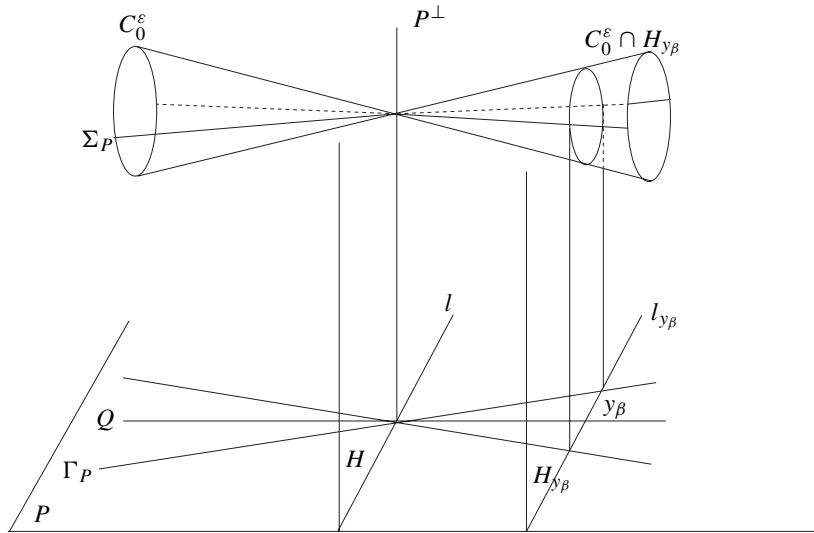
Figure 4. The case n = 2 and k = 1 .
