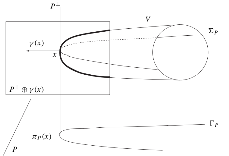
Figure 3. The index i_P(x) .
