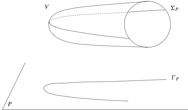
Figure 2. The sets \Sigma_P and \Gamma_P .
