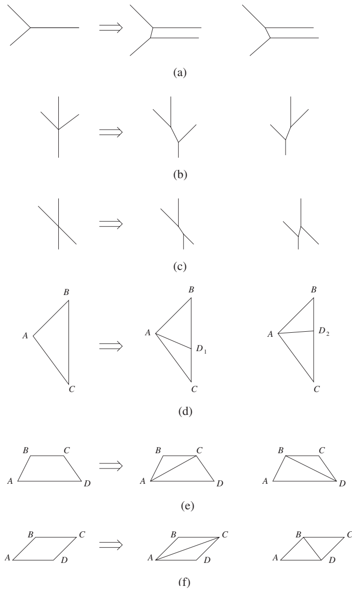
Figure 4. Degenerate second bifurcations.
