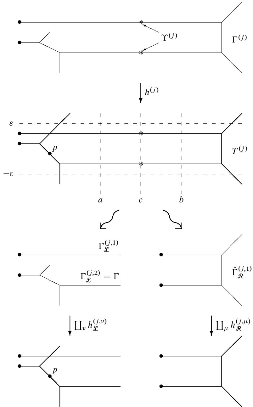
Figure 6. Cut in the proof of Theorem 3.
