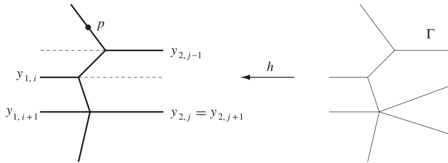
Figure 5. Curve (\Gamma, w, h) in Lemma 29.
