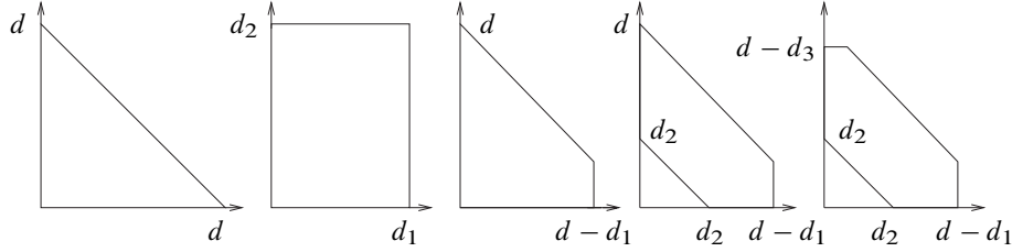
Figure 1. Polygons associated with Del Pezzo surfaces.
