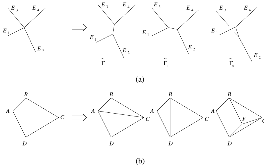
Figure 3. Non-degenerate second bifurcation.
