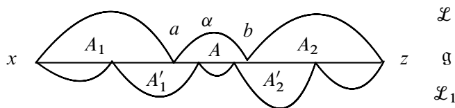
Figure 4. Step 1 in the proof of Lemma 4.18.
