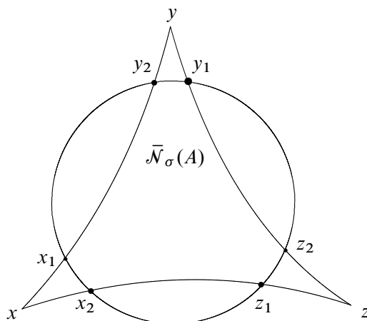
Figure 5. Case (P) of Definition 4.27.
