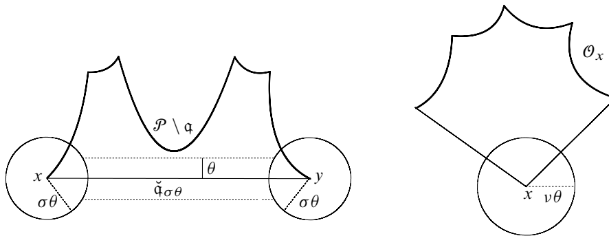
Figure 3. Properties (Fat 1 ) and (Fat 2 ).
