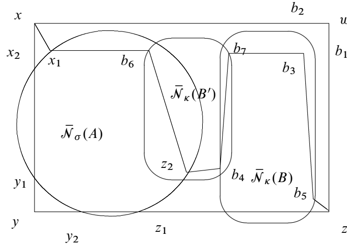
Figure 7. Case 2.B in the proof of Lemma 4.33.
