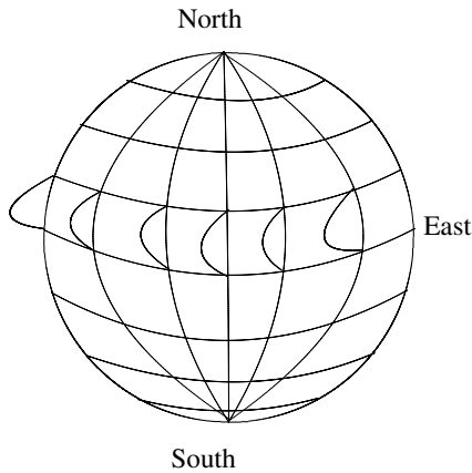
Figure 1. The graph \Gamma_k .
