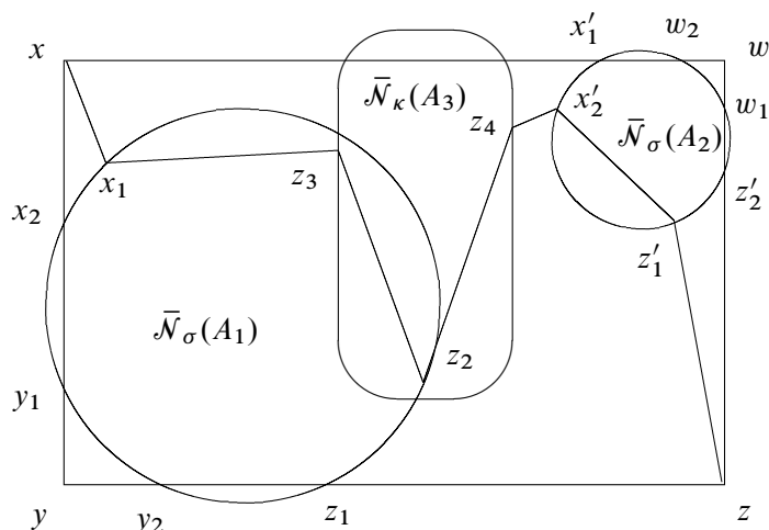
Figure 8. Case 3 in the proof of Lemma 4.33.
