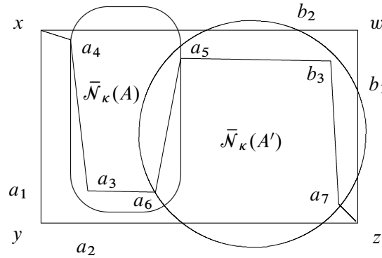
Figure 6. Case 1 in the proof of Lemma 4.33.
