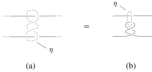
Figure 4.2. Isotopy of K \cup \eta .
