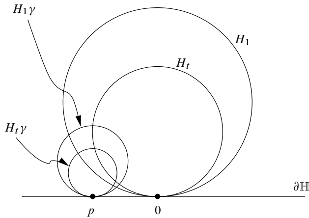
Figure 1. Intersection of horocycles.
