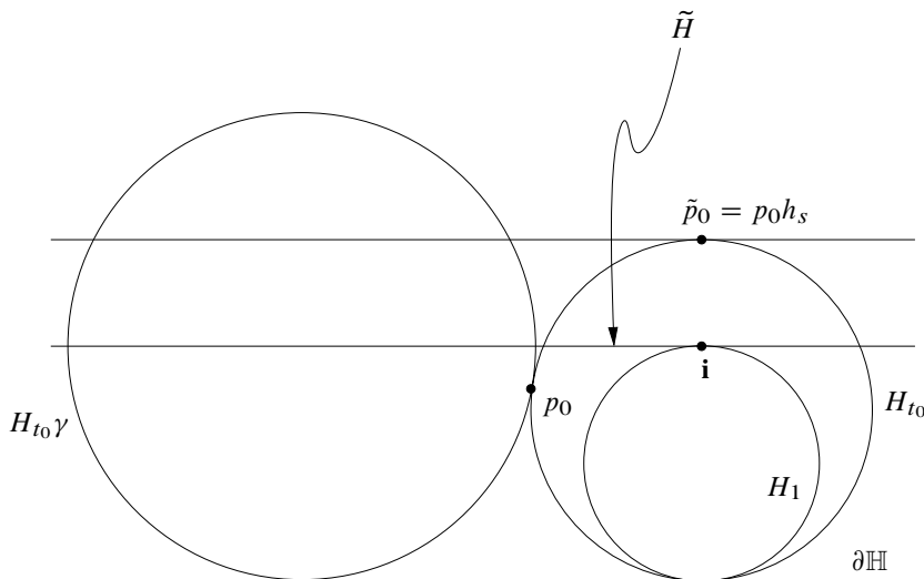
Figure 2. Tangency of H_{t_0} and H_{t_0}\gamma .
