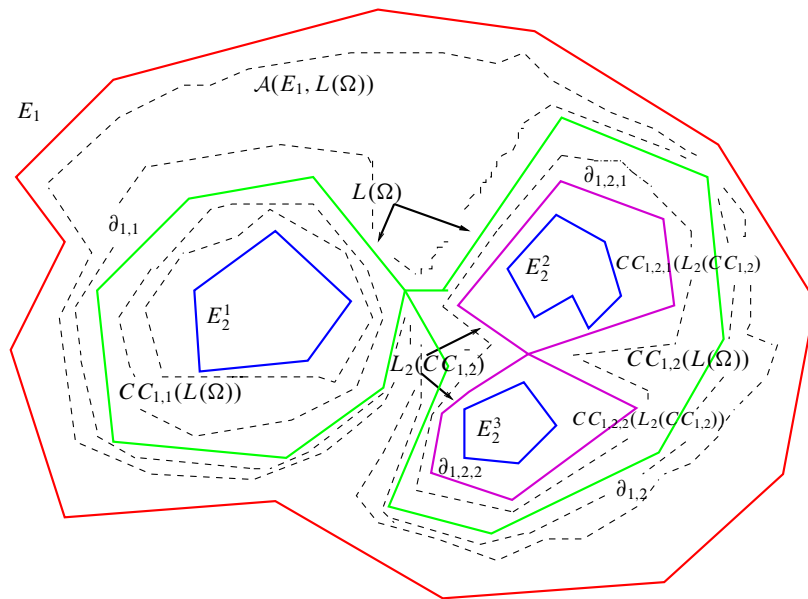
Figure 6.6. An example of a splitting scheme.
