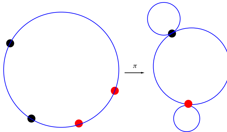
Figure 5.20. An example of the map \pi .
