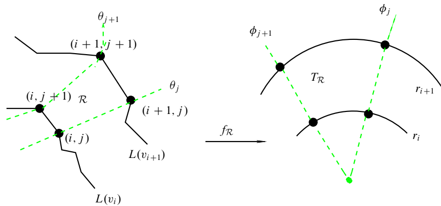
Figure 5.9. Constructing one annular shell.
