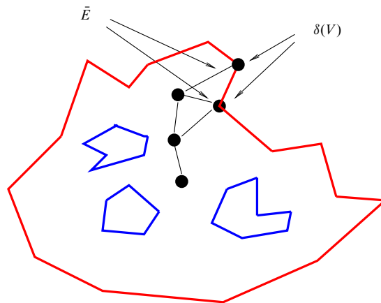
Figure 2.4. An example where V consists of all the vertices in the topological interior.
