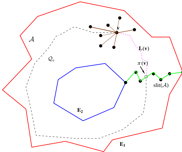
Figure 3.2. An example of a quadrilateral Q_v .
