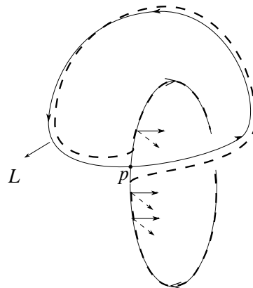
Figure 4. The dash line is the transversal \gamma . The dash and real arrows on the circle pointing outside give the orientations of \mathcal{G} and \mathcal{F} respectively.
