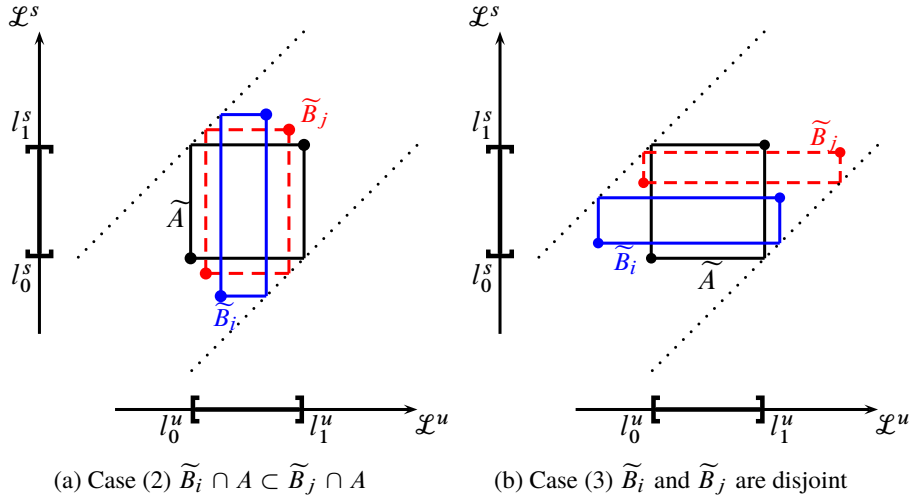
Figure 11. Possible types of intersections of the lozenges \tilde{B}_i (blue (mid gray)) and \tilde{B}_j (red (dark gray)) with \tilde{A} (black).
