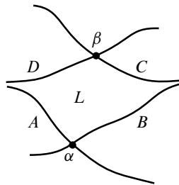
Figure 2. A lozenge with corners \alpha, \beta and sides A, B, C, D .
