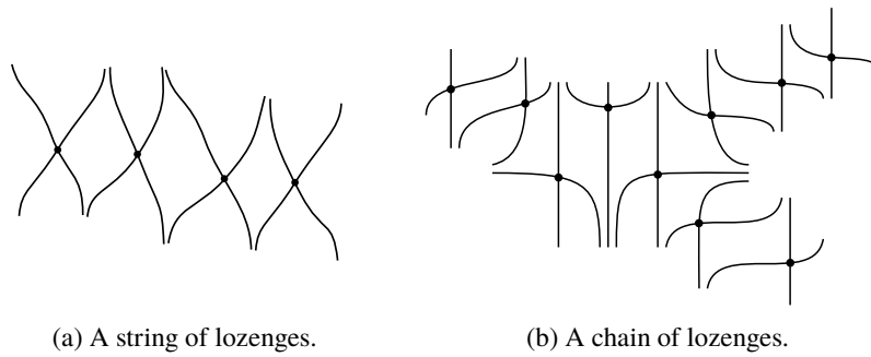
Figure 3. Chain and string of lozenges.
