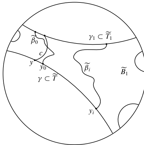
Figure 9. Large horizontal distance between y_0 and y_i .
