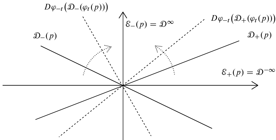
Figure 1. Configuration of lines in \mathcal{E}(p)/\mathcal{W}(p) .
