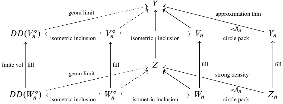
Figure 2. The manifolds appearing in the statement and proof of Theorem 7.2. Hooked horizontal arrows represent isometric inclusions. Dashed horizontal lines represent a small quasi-conformal deformation that produces a circle-packed manifold. Vertical arrows represent Dehn filling. Solid diagonal arrows represent strong limits. Dashed diagonal arrows represent geometric limits only.
