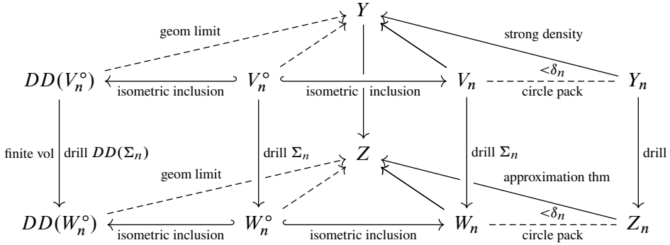
Figure 1. The manifolds appearing in the statement and proof of Theorem 6.2. Hooked horizontal arrows represent isometric inclusions. Dashed horizontal lines represent a small quasi-conformal deformation that produces a circle-packed manifold. Vertical arrows represent drilling out an embedded link. Solid diagonal arrows represent strong limits. Dashed diagonal arrows represent geometric limits only.
