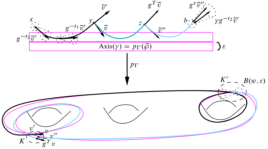
Figure 2. Connecting lemma.
