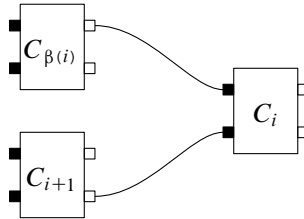
Figure 11. Connecting the Choi–Jamiołkowski matrices C_i by the permutation \beta and \gamma , where \gamma(i) = i + 1 .
