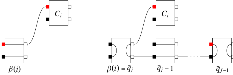
Figure 12. Following the top outputs (in red) of the C -boxes in the diagram \text{Tr}_{\beta, \gamma}[C_1^{\mathcal{Q}}, C_2^{\mathcal{Q}}, \dots, C_{n-1}^{\mathcal{Q}}, C_n] . Left: \beta(i) \notin \bar{\mathcal{Q}} ; right: \beta(i) = \bar{q}_j \in \bar{\mathcal{Q}} .
