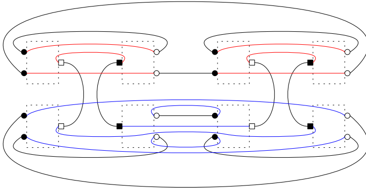
Figure 9. The diagram \mathcal{D}_{\alpha=(1)(2),\beta=(12)} as a term in the graphical Wick expansion of \mathbb{E} \operatorname{Tr} Z^2 . This diagram consists of 6 d -dimensional loops (3 corresponding to the top (red) pictures and 3 corresponding to the bottom (blue) ones) and of 1 \ell -dimensional loop.
