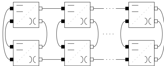
Figure 14. The diagram for \text{Tr}[\omega_\ell Z^{n-1}] . Each row contains (n - 1) boxes corresponding to the Choi–Jamiołkowski matrix of the map \Psi .
