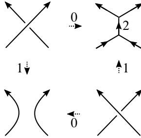
Figure 3. MOY graphs obtained by resolving crossings of an oriented link diagram. An edge of an MOY graph without an explicit label is labeled 1. The top left crossing is positive, and the bottom right crossing is negative.
