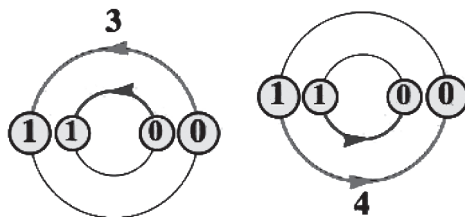
Figure 4. The morphism \psi : \mathfrak{g}(1) \rightarrow \mathfrak{g}(1) has module 8, it gives a map F_{\psi} : F_x \rightarrow F_{F(8)x} \cong \text{Sd}_8^*(F_x) .
