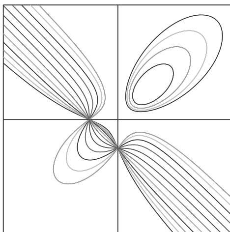
FIGURE 1 The Hesse pencil
