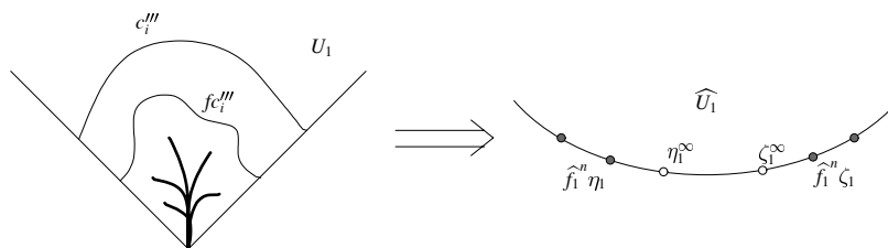
FIGURE 13 No topological chain \{c_i'''\}
