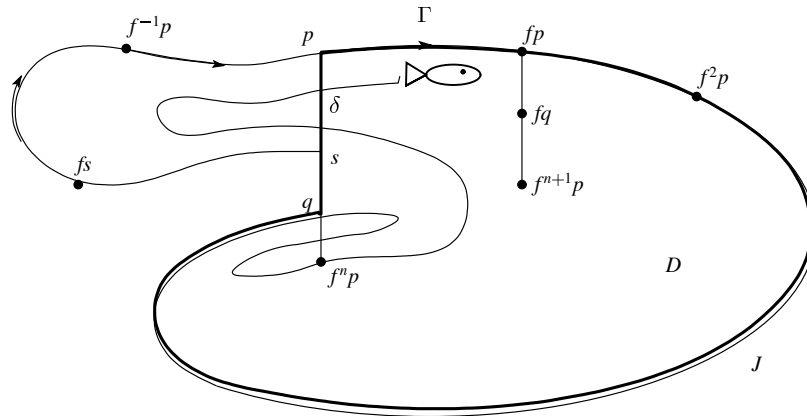
FIGURE 16 The curve J
