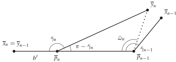
FIGURE 3 Constructing \bar{H}_n from \bar{H}_{n-1}
