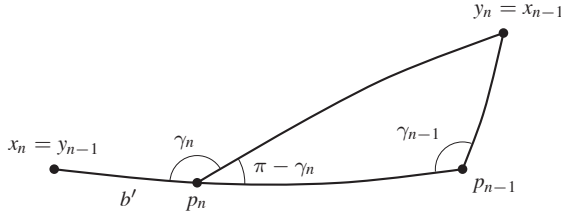
FIGURE 2 Constructing H_n from H_{n-1}
