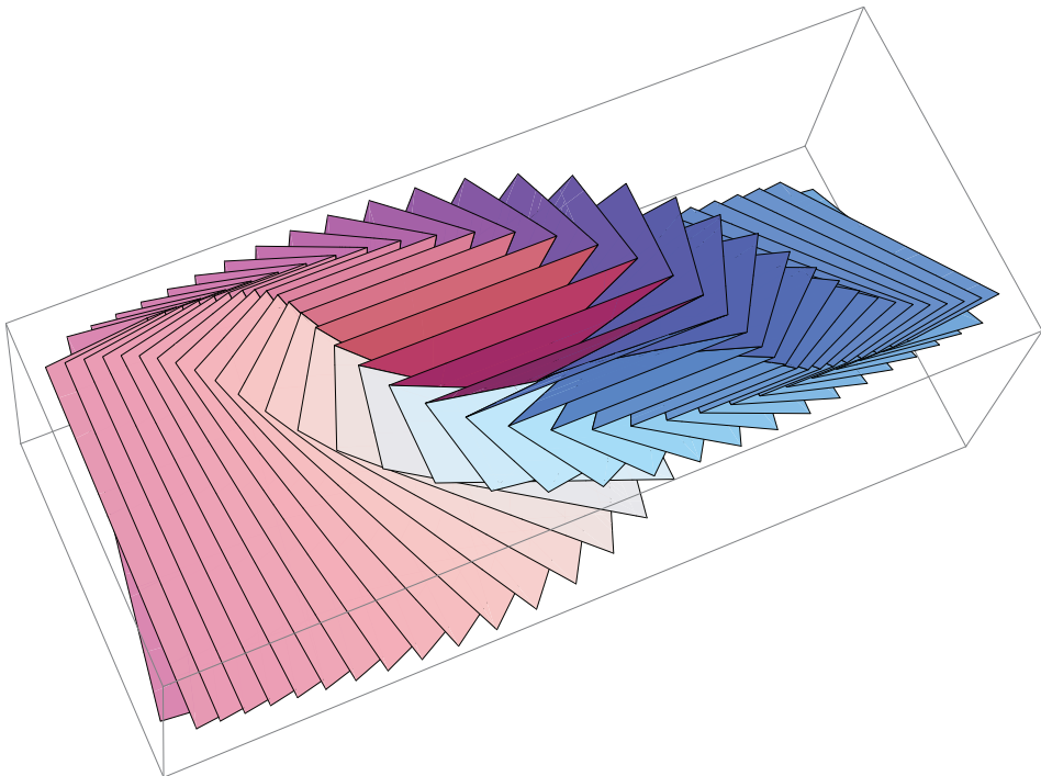
FIGURE 7 A crooked foliation
