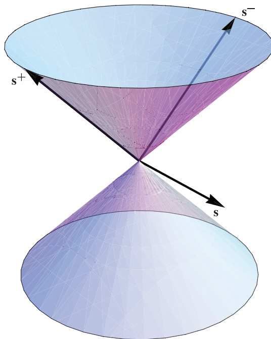
FIGURE 2 A null frame
