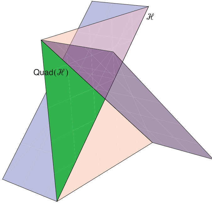
FIGURE 4 The stem quadrant of a crooked halfspace
