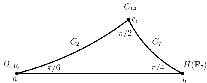
FIGURE 2 The vertex and edge groups in E(\mathcal{Y})
