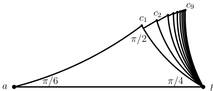
FIGURE 1 The complex \mathcal{Y}
