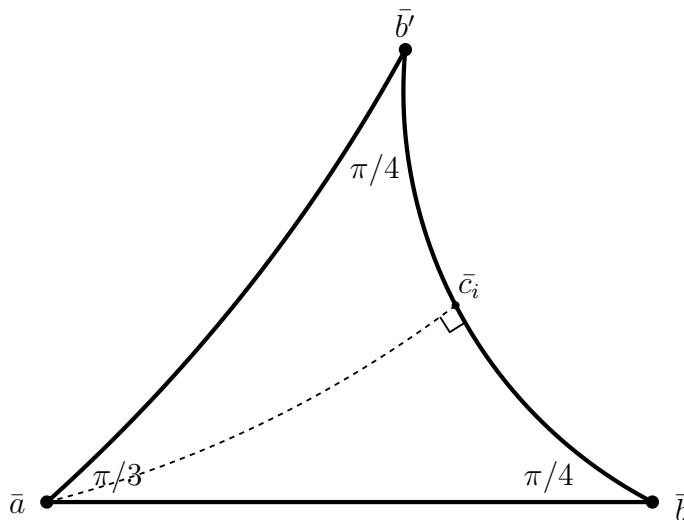
FIGURE 3 Discarding the thin edges
