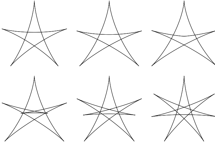
Fig. 7a Caustics of tables with \rho(\alpha) = a_0 + g \cos(5k\alpha) + (1 - g) \cos(7k\alpha) for g = k/7 , k = 1, \dots, 6 . We see an interpolation between the caustics with 5-fold and 7-fold symmetry in Figure 6a.
