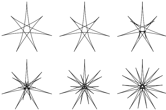
Fig. 7b Examples of caustics obtained from tables determined by \rho(\alpha) = a_0 + g \cos(7k\alpha) + (1 - g) \cos(17k\alpha) for g = k/7 , k = 1, \dots, 6 . We see an interpolation between caustics with 7-fold and 17-fold symmetry.
