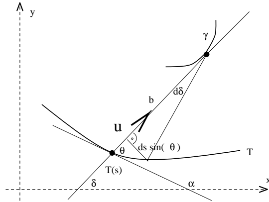
Fig. 5 The relation b(s) = \sin(\theta)(d\delta/ds)^{-1} in the proof of Lemma 3.1. When inserting this relation into the formula \gamma = T + bu , it gives the formula for the caustic \gamma in terms of the table T and the invariant curve \Gamma in the phase space.
