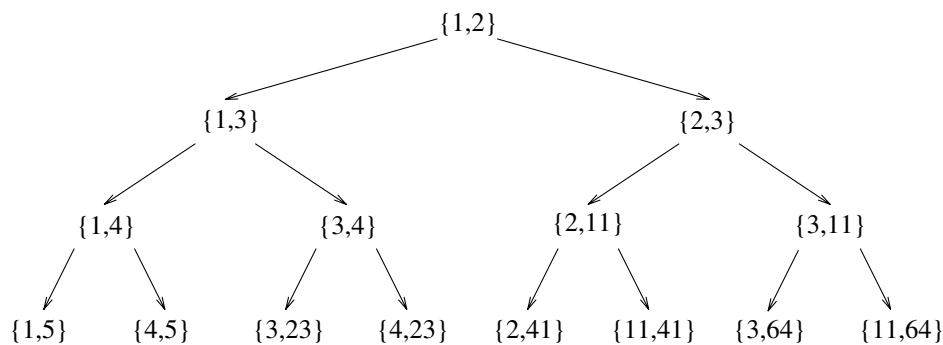
Fig. 1 Applying Algorithm 2.
