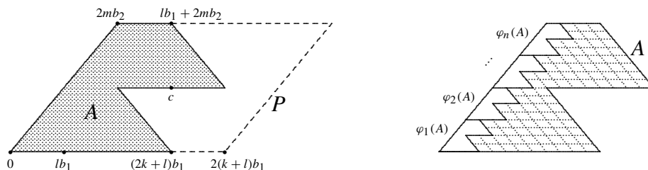
Fig. 4 Proof of Proposition 2
