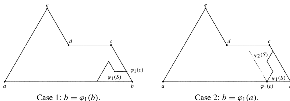
Fig. 7 Proof of Proposition 4
