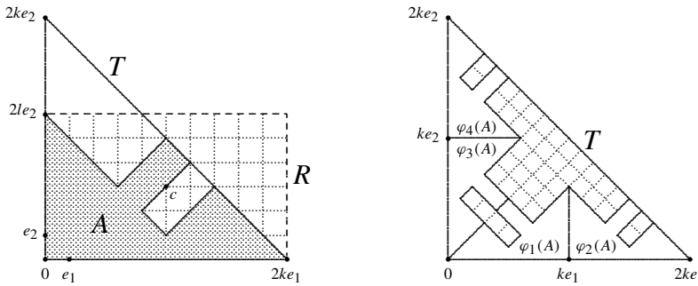
Fig. 8 Proof of Proposition 5
