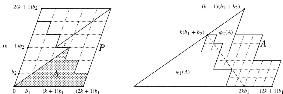
Fig. 9 Proof of Proposition 6
