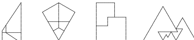
Fig. 2 Examples of irreptiles (see [9])
