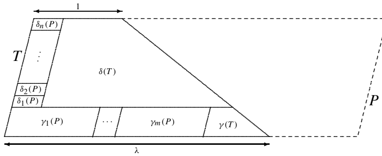
Fig. 14 Proof of Proposition 9
