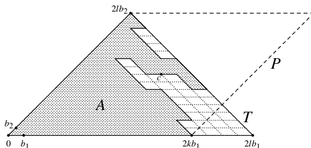
Fig. 3 Proof of Proposition 1
