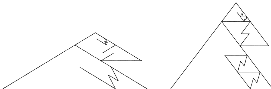
Fig. 12 Two non-lattice examples
