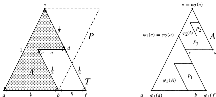
Fig. 11 Proof of Proposition 8
