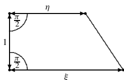
Fig. 13 The trapezoid H(\xi, \eta)
