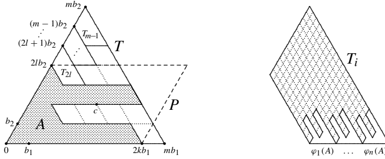
Fig. 5 Proof of Proposition 3
