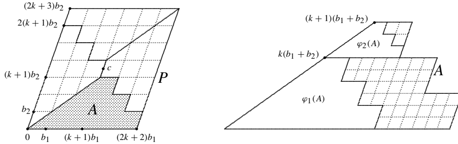
Fig. 10 Proof of Proposition 7
