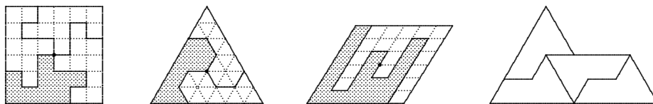
Fig. 1 Examples of reptiles
