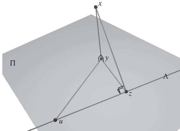
Fig. 1 Equivalence between Theorem 0 and Variant I.
