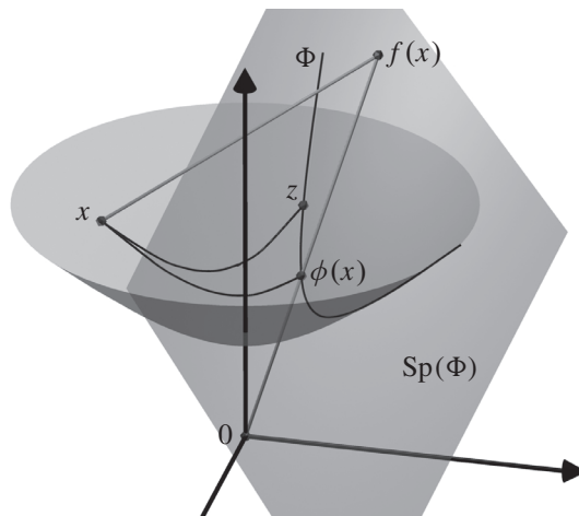
Fig. 4 Metrical projection on hyperbolic spaces.
