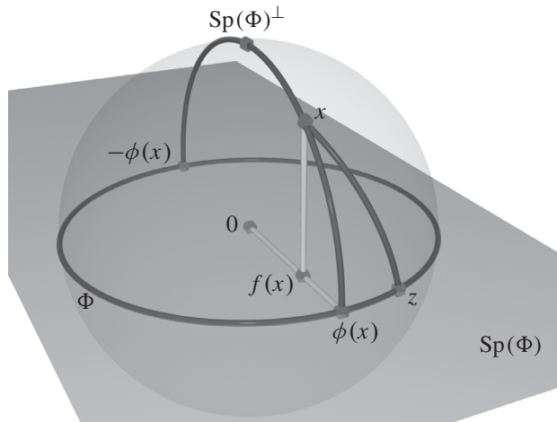
Fig. 2 Metrical projection on spheres.
