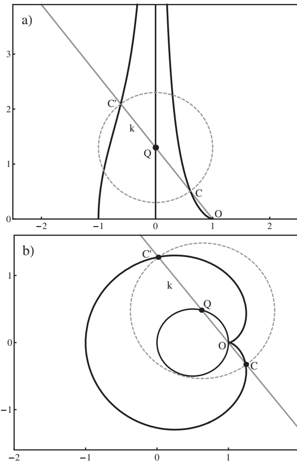
Figure 3 The defining properties of the conchoid of Nicomedes and the cardioid are present in the Axiata A^i(x) and A^e(x) respectively. In both a) and b) we have CQ = C'Q = k , for any straight line passing through O .
