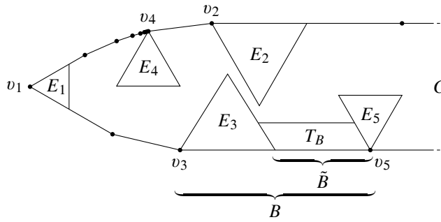
Figure 3 Proof of Proposition 8
