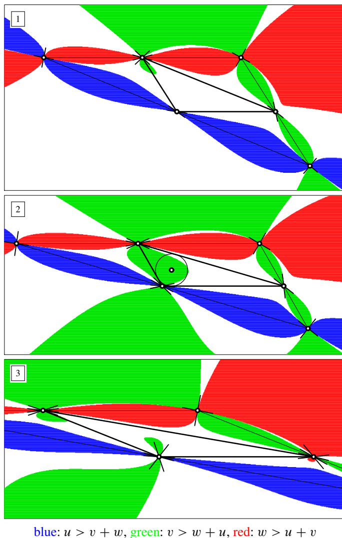
Figure 3. Triangles with 1, 2, and 3 double “forbidden” sectors; little tracts indicate the asymptotic directions (1) and (2). A = (-1, 0) , B = (1, 0) , \boxed{1} : C = (-1.7, 1.1) , \boxed{2} : C = (-1.4, 0.7) , \boxed{3} : C = (-2.5, 0.6)
