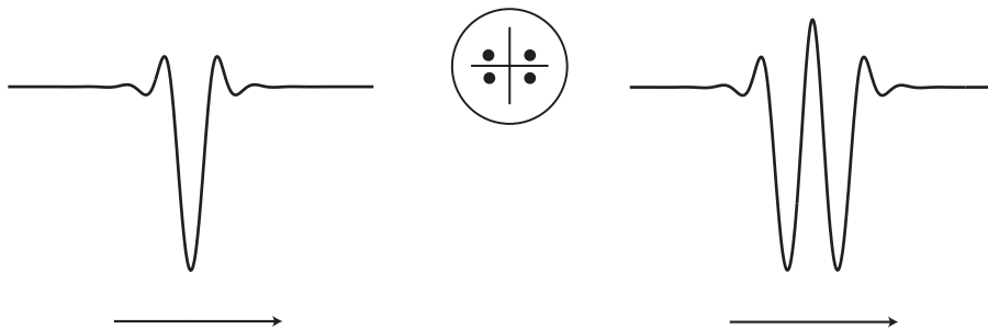
FIGURE 2. Two of the multi-trouged solitary waves found by B. Buffoni, M. D. Groves & J. F. Toland on a four-dimensional invariant manifold with the depicted eigenvalue structure.
