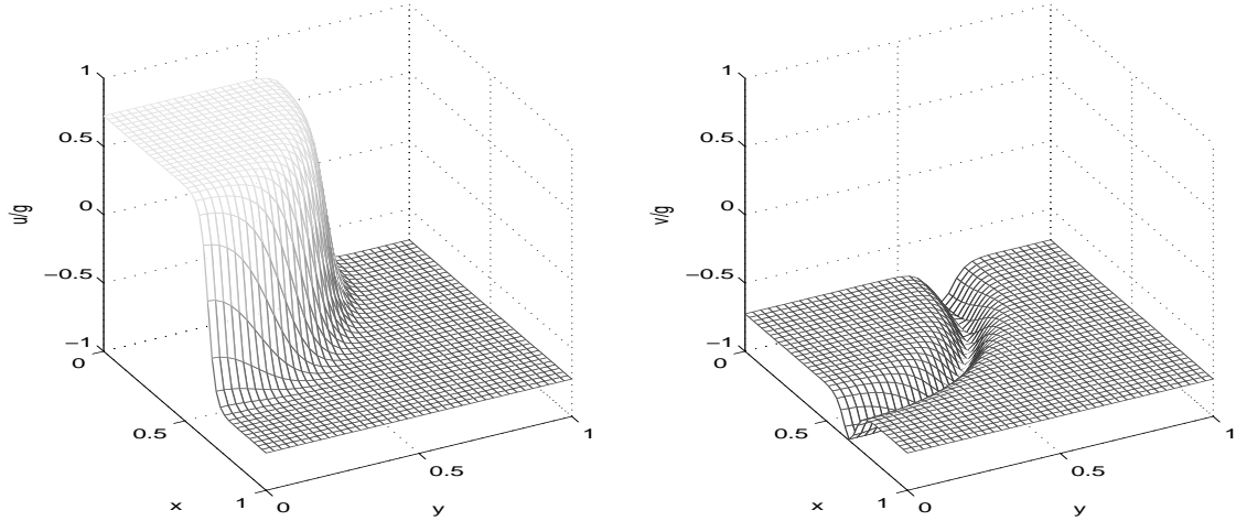
FIGURE 6. Steady solutions to problem (P) , with \Omega = (0,1) \times (0,1) , \alpha = 0.9 , \epsilon = \frac{1}{200} , f \equiv k \equiv 1 , and g(x,y) = \begin{cases} 1 - 3 \cosh(\pi r)^2 \exp(-\frac{1}{1-r}) \exp(-\frac{1}{r}) & \text{if } r := \sqrt{x^2 + y^2} \leq 1; \\ 1 & \text{otherwise.} \end{cases} (Steady limit of a numerical simulation of the time-dependent gradient system showing that these local minimisers act as stable attractors for a wide range of initial data with appropriate sign changes.)
