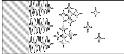
FIGURE 1. Columnar (left) and equiaxed (right) dendritic structures
