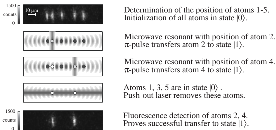
FIGURE 1. Quantum Register with 5 Caesium Atoms. The images were taking with a photon counting camera. Resolution is about 1 \mu\text{m} per pixel.
