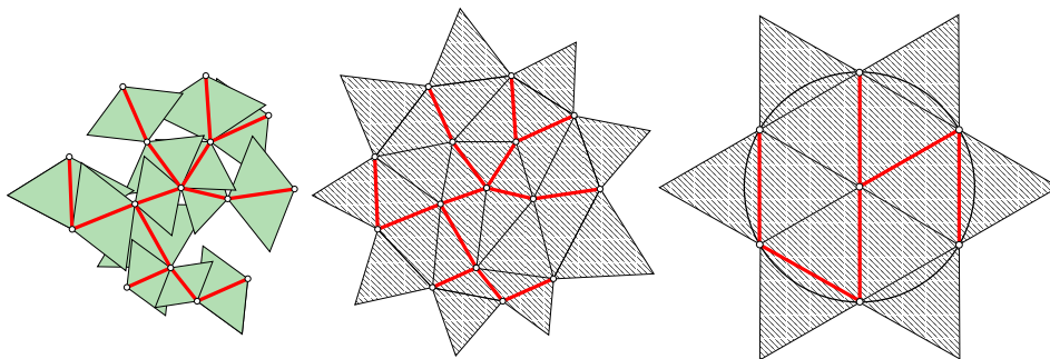
FIGURE 1. The total area of the equilateral triangles on the left is bounded by the hatched area in the middle. The point set that maximizes the hatched area is shown on the right.
