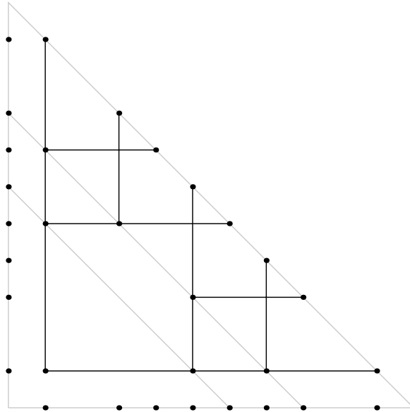
FIGURE 1. If the sumset is small, then the Cartesian product, A \times A , can be covered by using only a few lines of slope -1 . Select one, which covers the most points of the Cartesian product. Consider the points lying on this line and the smaller Cartesian product defined by these points. Repeat the process, until the most popular line with slope -1 contains only one point of the last Cartesian product. Going back from this point along the nested Cartesian products we get a binary tree. It is easy to check that the projection of the tree onto the horizontal (or vertical) line determines an affine cube in A .
