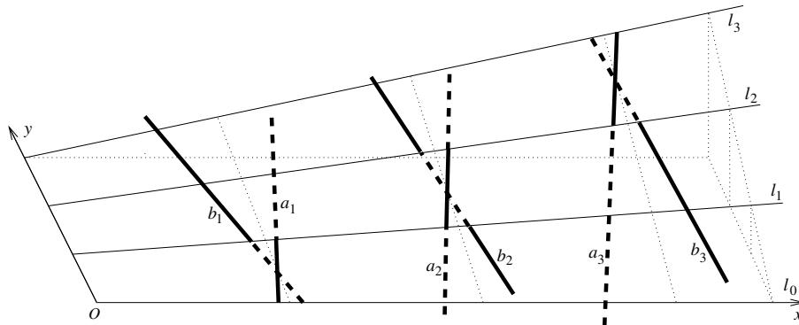
FIGURE 1. The segments a_i and b_i , for n = 3 .
