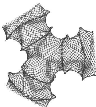
FIGURE 3. Hoffman Discrete K-Surface
