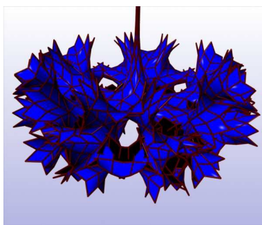
FIGURE 2. Henderson-Taimina-Thurston Discrete K-Surface
