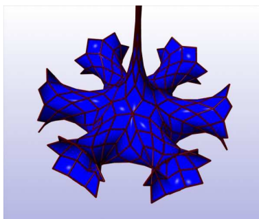
FIGURE 4. Hoffman-Sterling Discrete K-Surface
