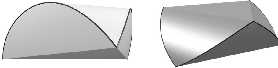
FIGURE 1. Convex surfaces glued from two Euclidean pieces identified along the boundary. Left : Disc and equilateral triangle. Right : Two Reuleaux triangles (triangles of constant width); the vertices of one are identified with the midpoints of the sides of the other.
