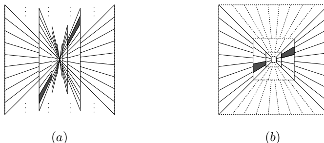
FIGURE 1. The tiling of the frequency domain induced by the discrete shearlets (a) and the discrete shearlets on the cone (b).
