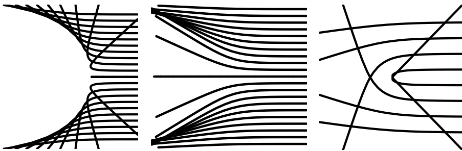
FIGURE 1. 2D scattering with degrees 1 (left), 0 (center) and -1 (right)
