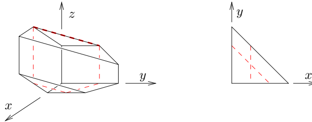
FIGURE 2. The projections P_{xyz} and P_{xy}
