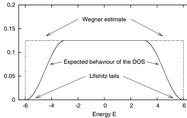
FIGURE 1. A schematic diagram summarizing the known results and the physical expectations with respect to the density of states of one energy band.
