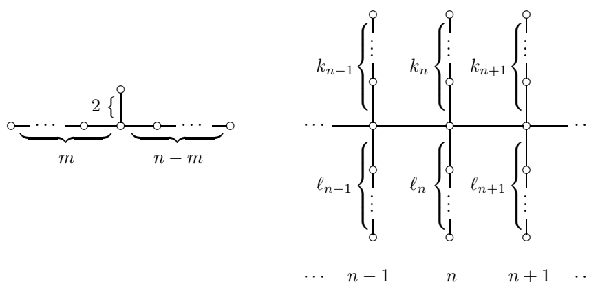
FIGURE 1. Dynkin diagrams T_{2,m,n-m} and T_\ell^k
